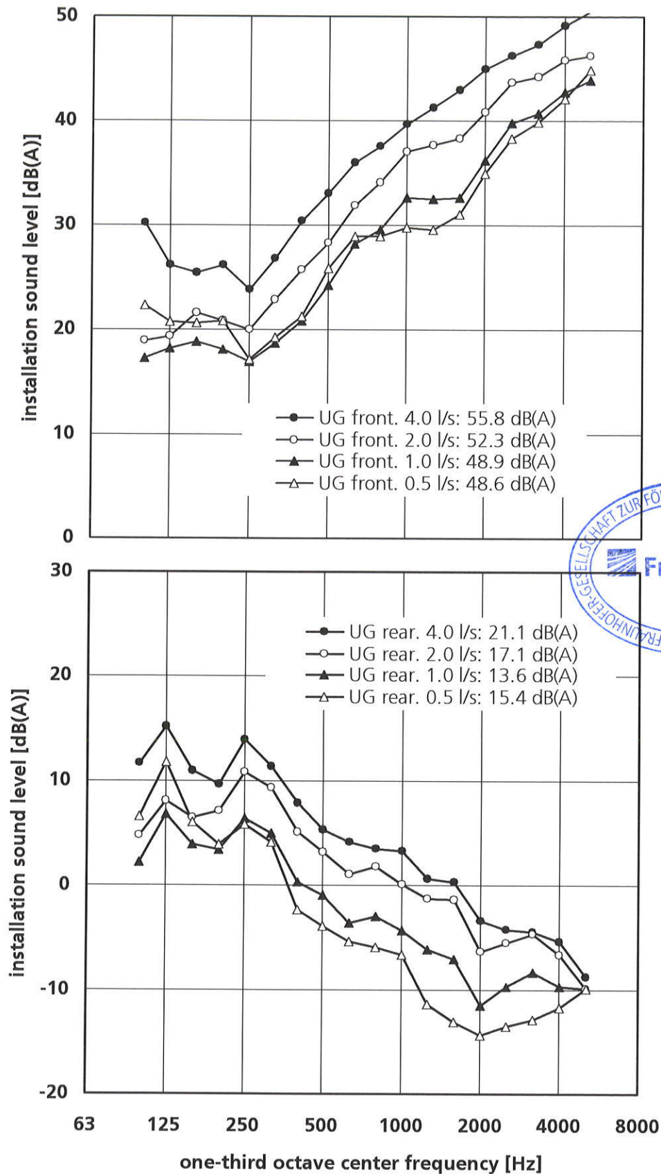
Figure 1 Wastewater pipe system "POLIphon" mounted in sub-basement (KG), basement (UG front), ground floor (EG front) and top floor (DG) using pipe clamps "POLIclamp". The installation sound level L_{in} was measured at various flow rates in the test rooms UG front (above) and UG rear (below).
