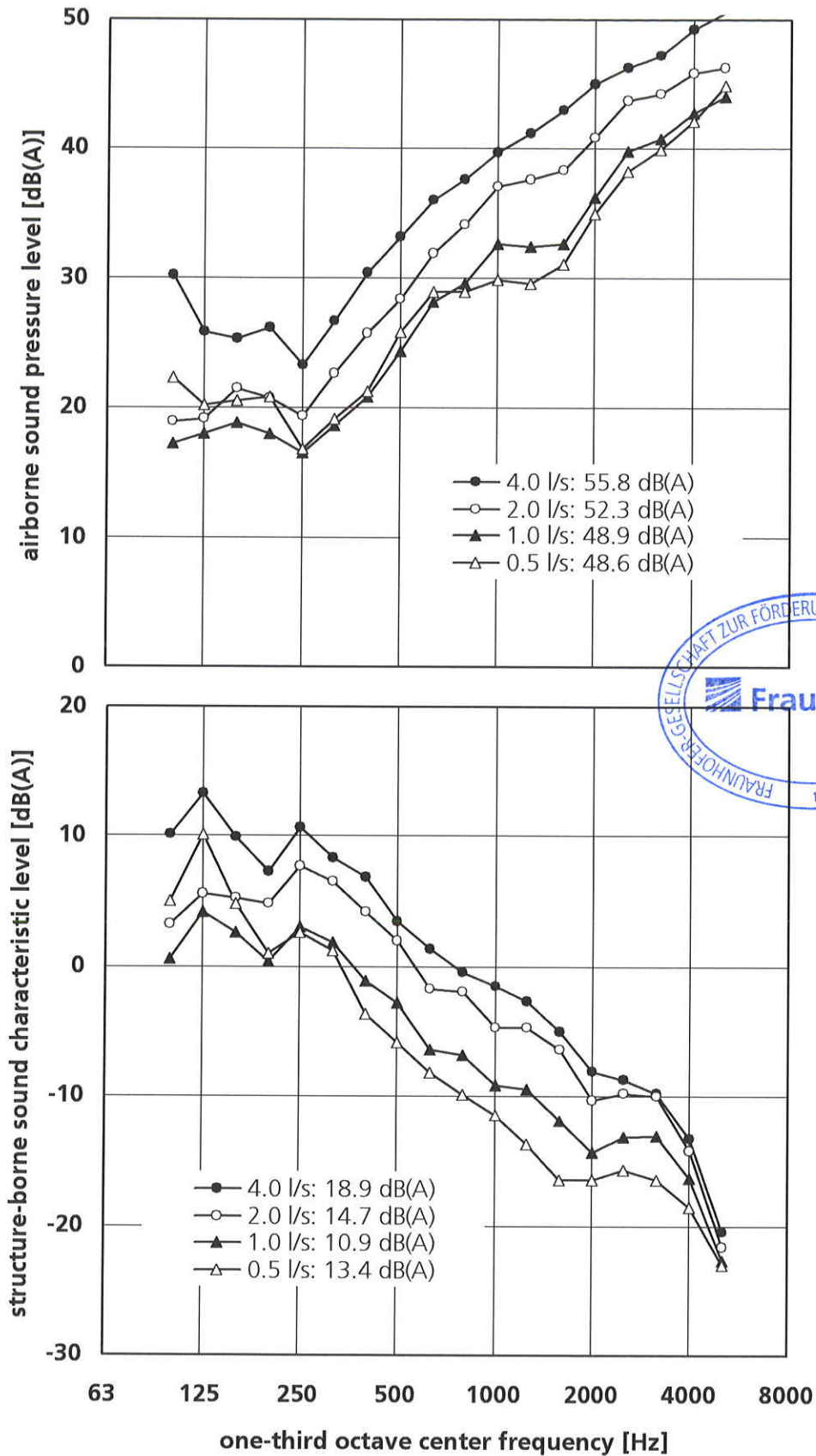
Figure 2 Wastewater pipe system "POLIphon" mounted in sub-basement (KG), basement (UG front), ground floor (EG front) and top floor (DG) using pipe clamps "POLIclamp". Airborne sound pressure level (above) and structure-borne sound characteristic level (below) measured at various flow rates according to DIN EN 14366.
