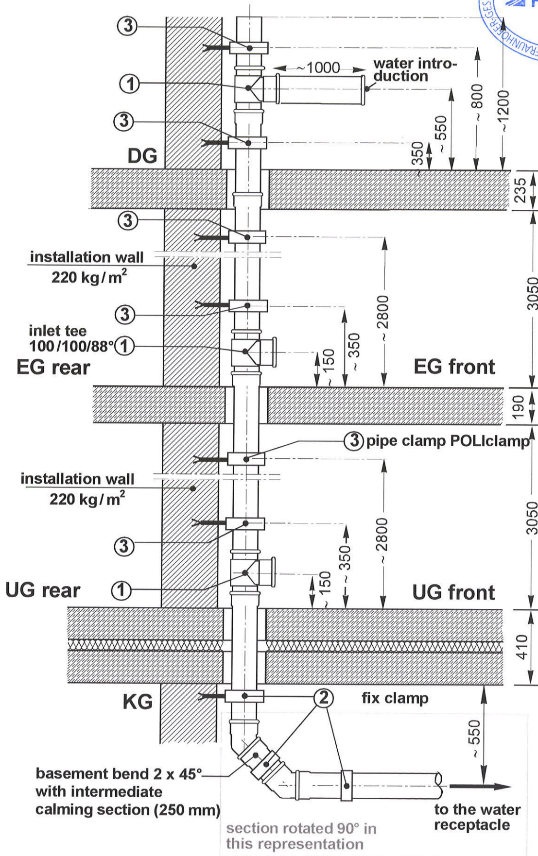
Figure 4 Installation plan of the pipe system "POLIphon" (manufacturer: Poliplast), mounted with clamps "POLIclamp" (drawing not to scale, dimensions in mm).
